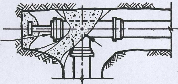
PLUGGED TEE
