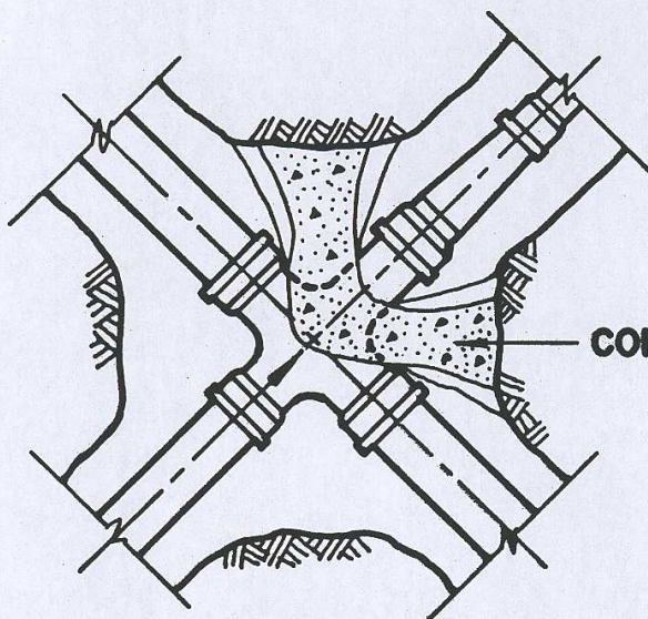
REDUCING CROSS
